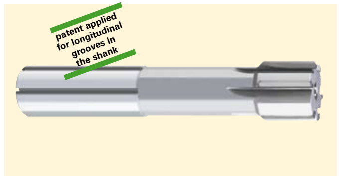
Cermet-tipped high-performance reamers HR 500 GD for the machining of through holes, Guhring no. 1683
